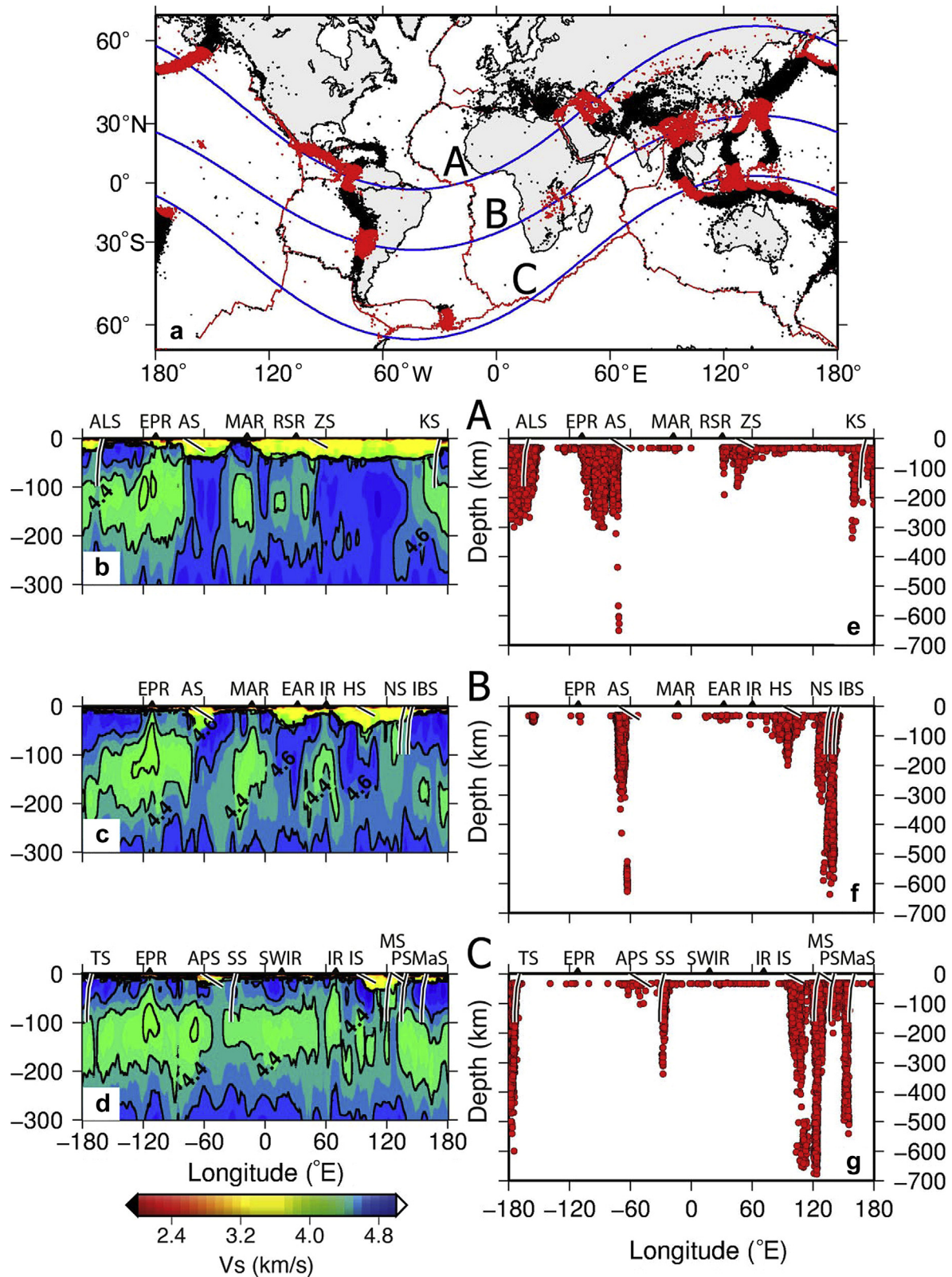
Figure 5. (a) Global seismicity from NEIC database at depth > 30 km ( http://earthquake.usgs.gov/regional/neic/ ) with lines B, A, C corresponding to the tectonic equator and its related 30^{\circ}\text{N} and 30^{\circ}\text{S} small circles respectively. The cross-section diagrams (b), (c), (d), along the circles A, B, C respectively, represent the values of the shear waves velocities ( V_s ) after Shapiro and Ritzwoller (2002). The western limbs of rift zones have in average a deeper bathymetry with respect to the eastern ones, and that, except for section (b), an approximately continuous low velocity layer 100–200 km can be detected in the upper asthenosphere. The cross-section diagrams (e), (f), (g), along the circles A, B, C respectively, show earthquake depth and represent the red points of (a). Beneath rift zones, earthquakes occur at lower depths, whereas under subduction zones an asymmetry is detected showing continuous seismicity as far as 670 km for W-directed subductions and the presence of a deeper scattered cluster of hypocentres between 550 and 670 km for E- and NE-directed subductions. Acronyms are those of Fig. 4.
