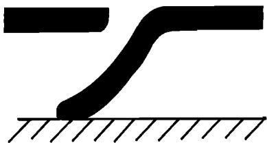
Fig. 14b. Lithosphere is deformed along its lower edge as it encounters a more resistant layer (the mesosphere).
